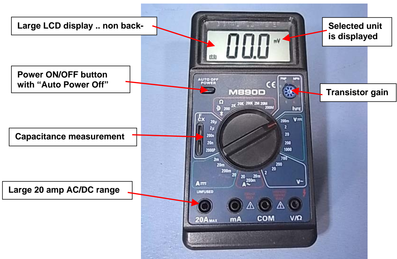
LB2124-001 digital multimeter
