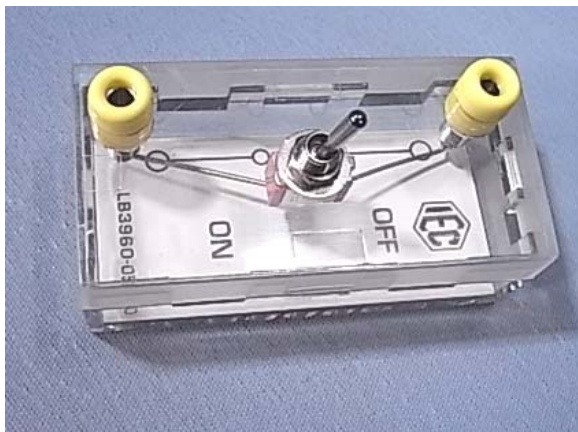
LB3960-050 SPST switch
